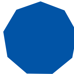
Nonagon
