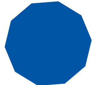
Decagon
