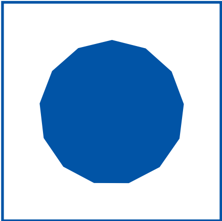
tridecagon
