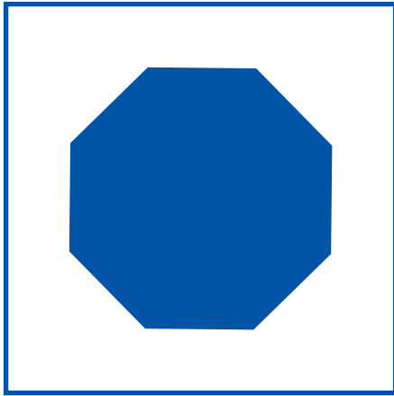
octagon
