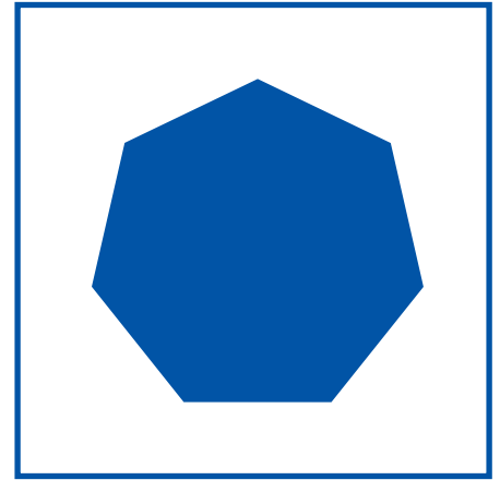
heptagon
