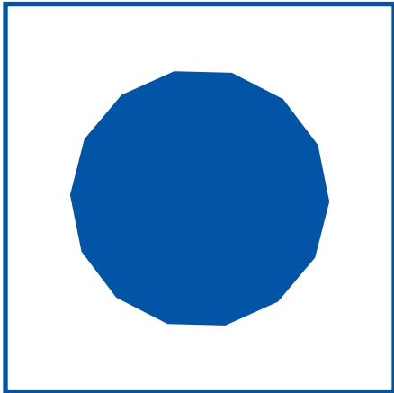
tetradecagon
