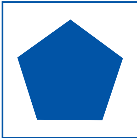
pentagon
