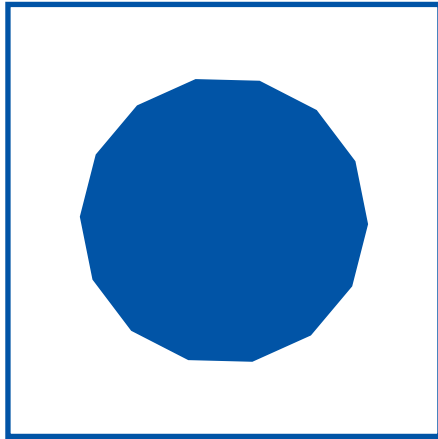
tetradecagon
