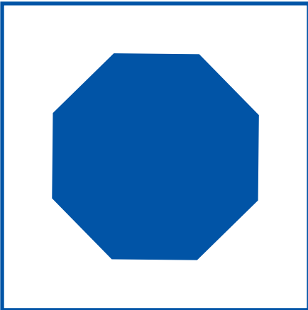
octagon
