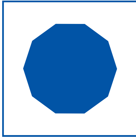
decagon
