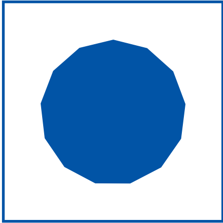
tridecagon
