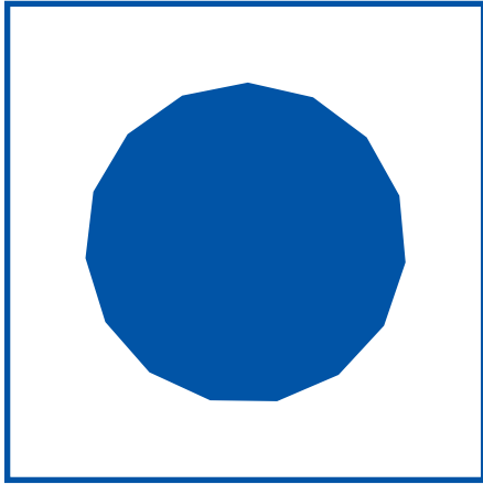
pentadecagon
