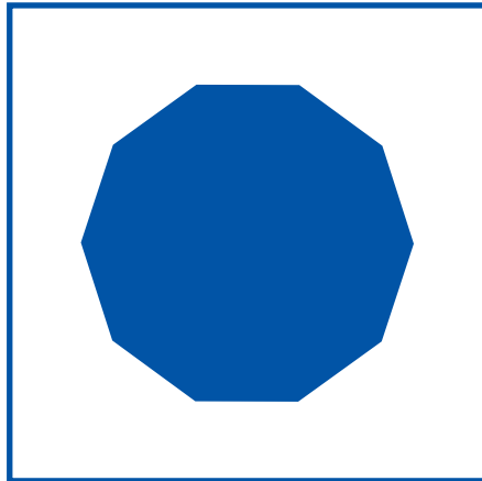
decagon
