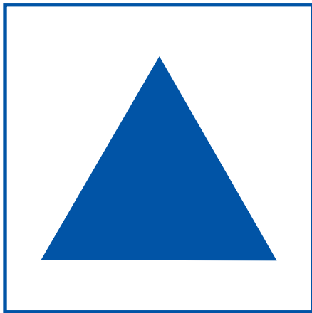
triangle
