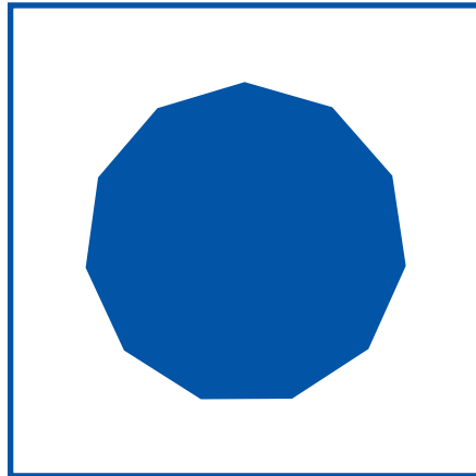
hendecagon
