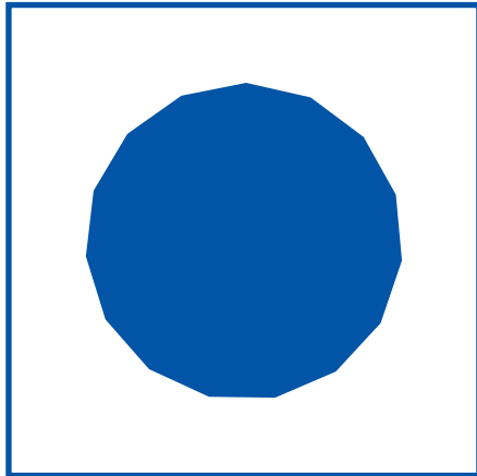
pentadecagon
