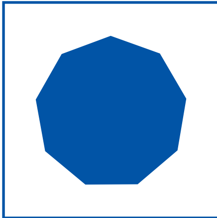
nonagon
