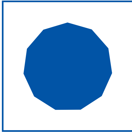
hendecagon
