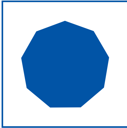
nonagon
