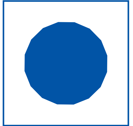
hexadecagon
