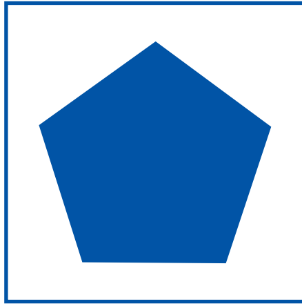
pentagon
